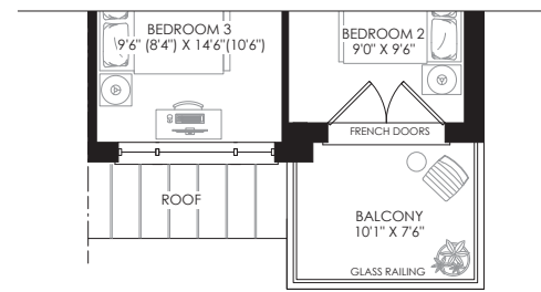
PARTIAL SECOND FLOOR PLAN ELEV. 'E'
