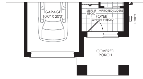
PARTIAL GROUND FLOOR PLAN ELEV. 'H','I'
