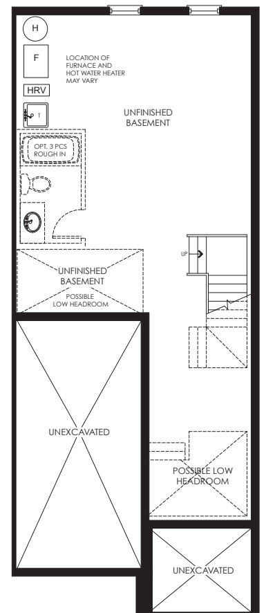
BASEMENT PLAN ELEV. 'D','E','H' & 'I'
