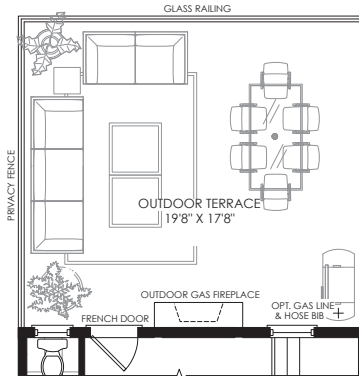
OPT. OUTDOOR FIREPLACE & DOOR LOCATION
