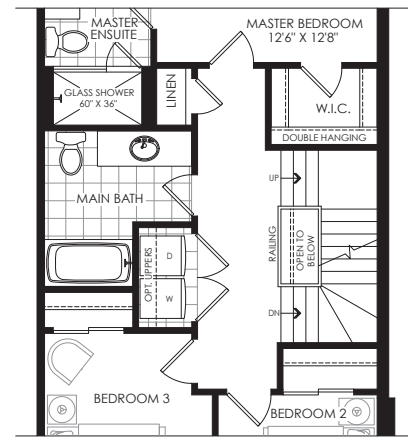
PARTIAL SECOND FLOOR FLEX PLAN WITH LAUNDRY
