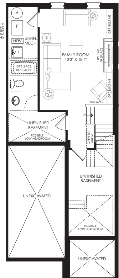
BASEMENT FLEX PLAN ELEV. 'D','E','H' & 'I'
