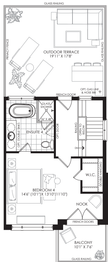
OPT. THIRD FLOOR PLAN ELEV. 'D' WITH BEDROOM 4
