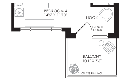
PARTIAL OPT. THIRD FLOOR PLAN ELEV. 'I' WITH BEDROOM 4
